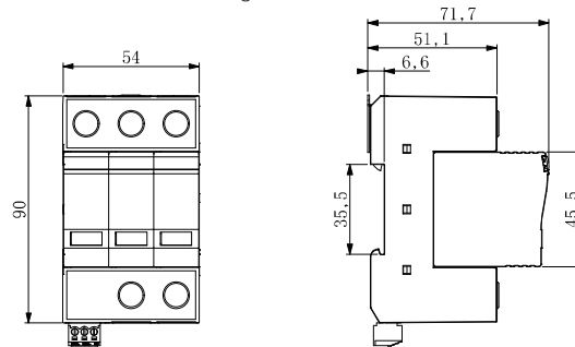
• Dimension drawing
