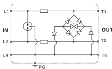
For 1-pair data line DM-...-M2N1
