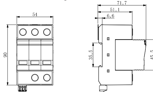
• Dimension drawing
