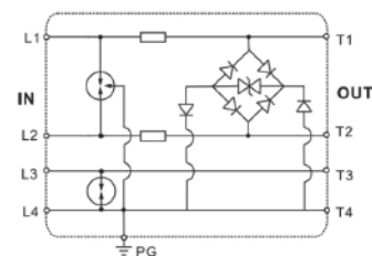
For 1-pair+shield data line DM-...-M2N3
